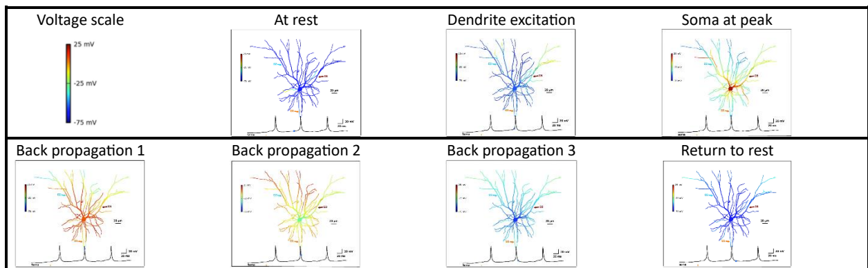
Figure 7. Back propagation of positive charge in a Level 2/3 neural action potential lasting \sim 20 msec
